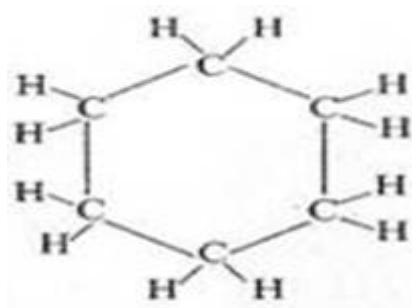
Cyclohexane
