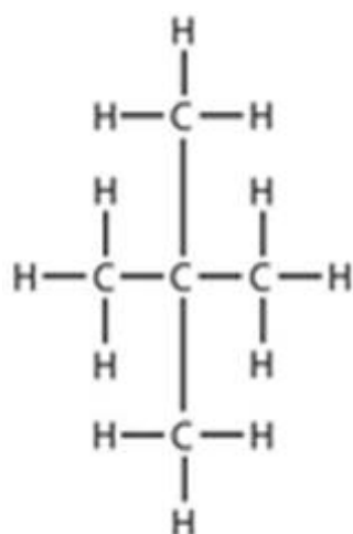
Neopentane
